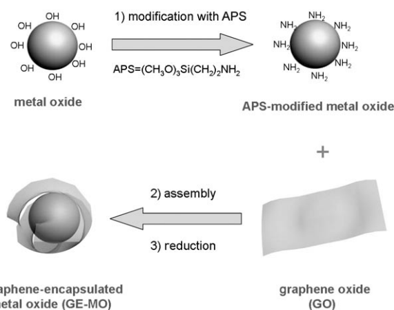
Figure 1. Fabrication of graphene-encapsulated metal oxide (GE–MO) including 1) modification of the metal oxide by grafting aminopropyltrimethoxysilane (APS) to render the oxide surface positively charged; 2) hybrid assembly between positively charged oxide nanoparticles and negatively charged graphene oxide by electrostatic interactions; and 3) chemical reduction.
